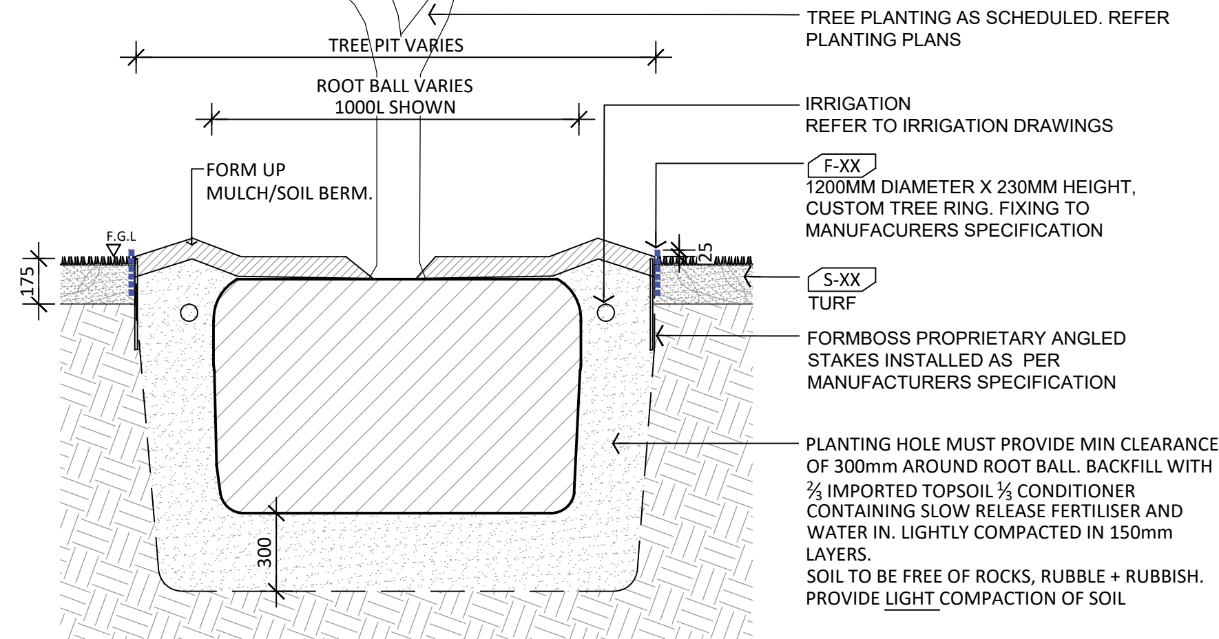
TREE - TURF TYP. SECTION DETAIL 1:20
