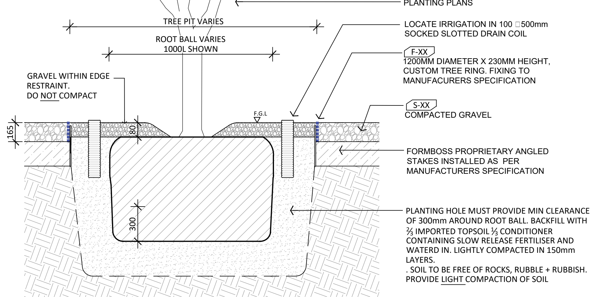
TREE - GRAVEL (TRAFFICABLE) TYP. SECTION DETAIL 1:20
