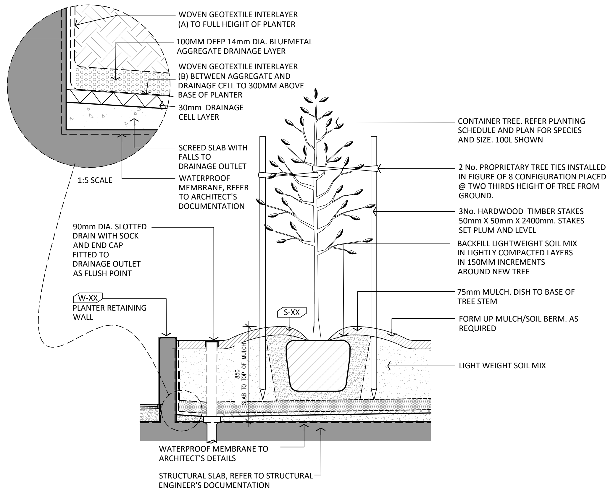
TREE - SLAB TYP. SECTION DETAIL 1:20
