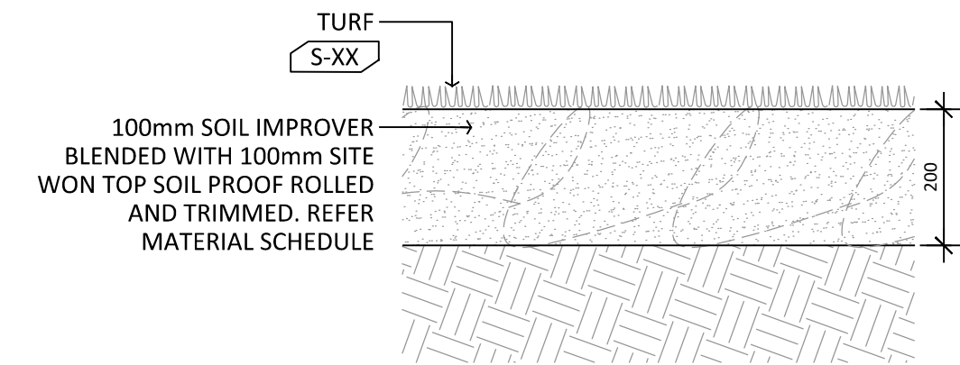
TURF - GROUND TYP. (SECTION) SECTION DETAIL 1:10
