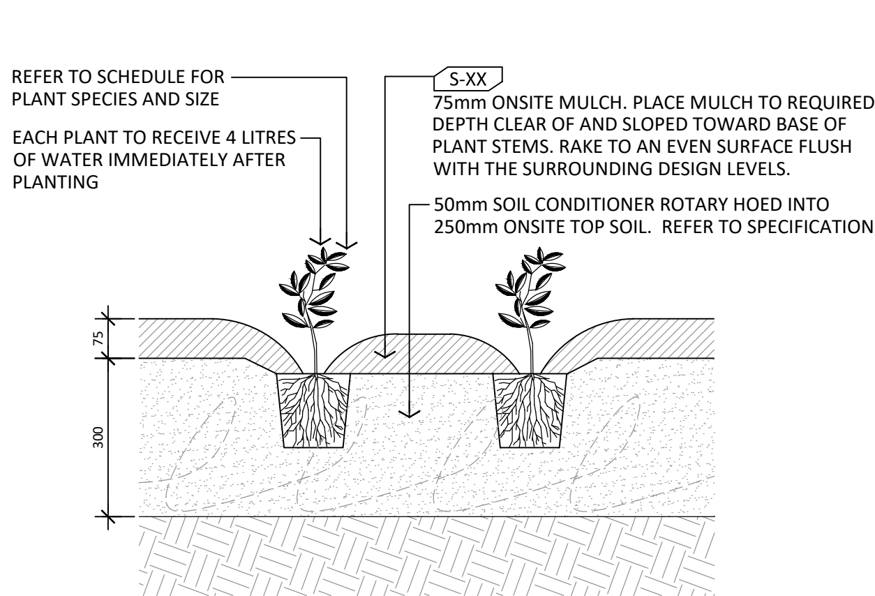
GARDEN BED - GROUND TYP. SECTION DETAIL 1:10
