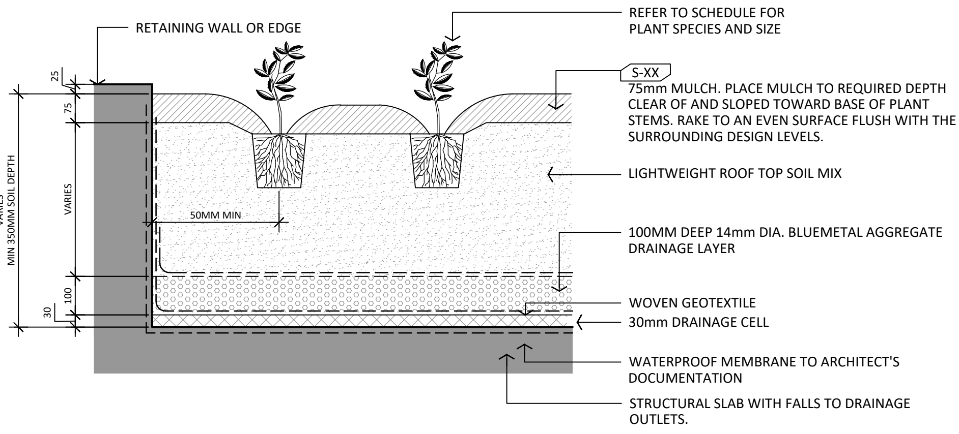
GARDEN BED - SLAB (INTENSIVE) TYP. SECTION DETAIL 1:10
