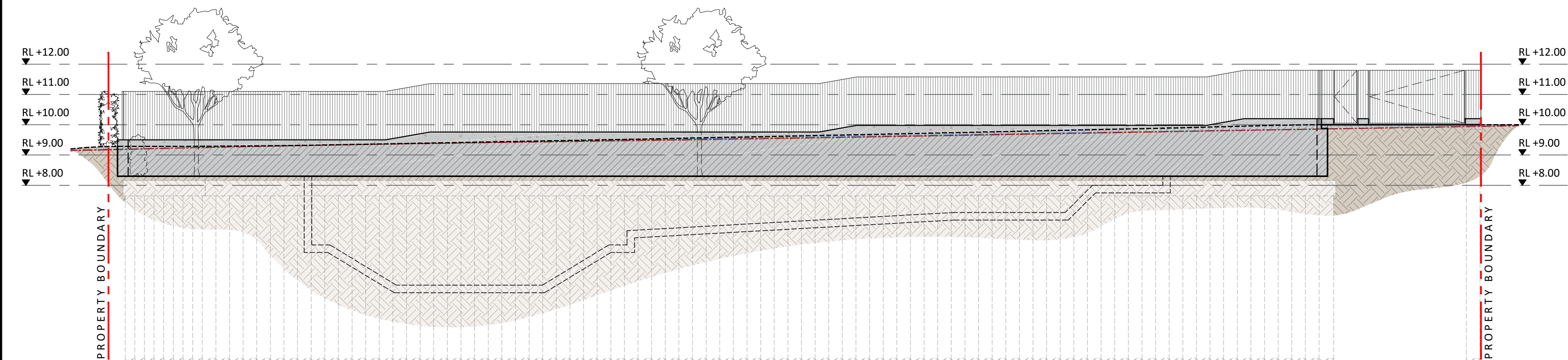
01 L-200 ROSENDO STREET ELEVATION ELEVATION 1:100
